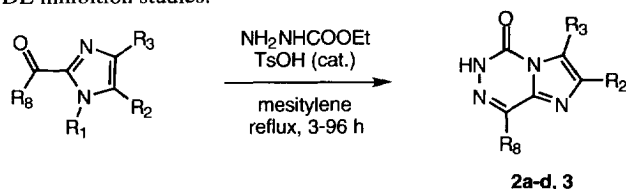
Scheme 1. Method A - R_1 = \text{H} . Method B - R_1 = \text{CH}_2\text{OCH}_3 .
