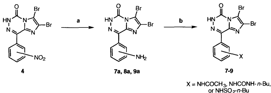
Scheme 2. Reagents and Conditions: (a), \text{SnCl}_2 , \text{HCl} , \text{H}_2\text{O} , \text{EtOH} , reflux, 4 h (60-85% yield). (b), \text{Ac}_2\text{O} , pyridine, rt, 1 h (80-82% yield); n\text{-Bu-NCO} , \text{DMF} , \text{CH}_3\text{CN} , reflux, 3-24 h (64-80% yield); or n\text{-BuSO}_2\text{Cl} , \text{Et}_3\text{N} , pyridine, rt, 16 h (48-57% yield).
